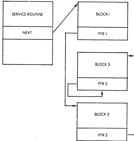
Fig. 9.5: A Queue
