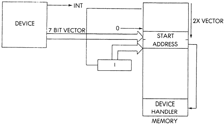
Fig. 6.29: Mode 2 Interrupt
