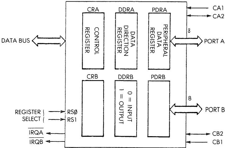
Fig. 7.1: Typical PIO
