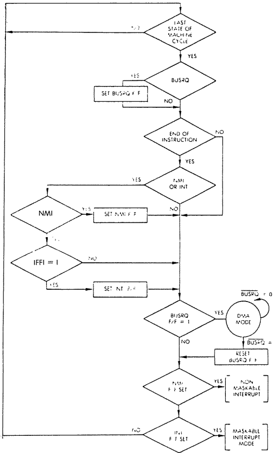
Fig. 6.24: Interrupt Sequence
