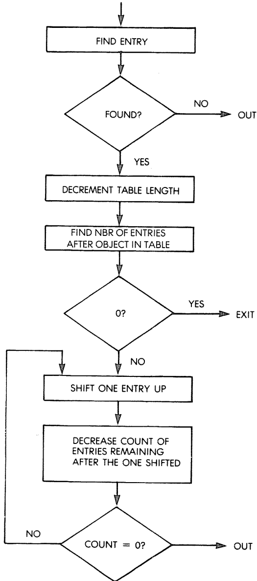
Fig. 9.15: Table Deletion Flowchart
