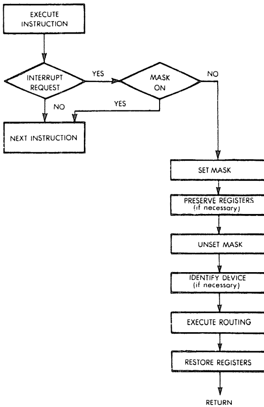
Fig. 6.34: Interrupt Logic
